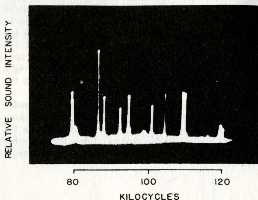
FIG. 2. Photograph of the cathode-ray screen of a panoramic ultrasonic analyzer, showing the frequency components occurring between 80 and 120 kc in a series of porpoise clicks. The separate pips represent the coincidence of the sweep of the cathode-ray tube with different clicks. The 12 clicks that occurred during the photographic exposure (.5 sec in this instance) thus contained frequencies extending at least to 120 kc.
