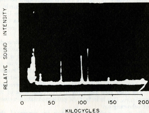
FIG. 3. Photograph of the cathode-ray tube of the panoramic analyzer when the tuning range was 10-200 kc. The strongest frequencies, so far as intensity is concerned, will be seen to lie below 25 kc, but the short pips at the right indicate the presence of frequencies at 140, 155, and 170 kc, respectively.
