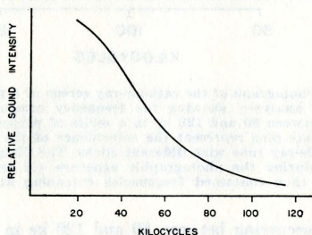
FIG. 4. Ultrasonic frequency spectrum derived from high-speed 4 tape recordings of the typical porpoise click. Essentially the same graph was obtained by two independent methods of acoustical analysis.
